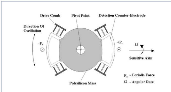
Fig. 1: Basic layout of the sensing element of SMG060
